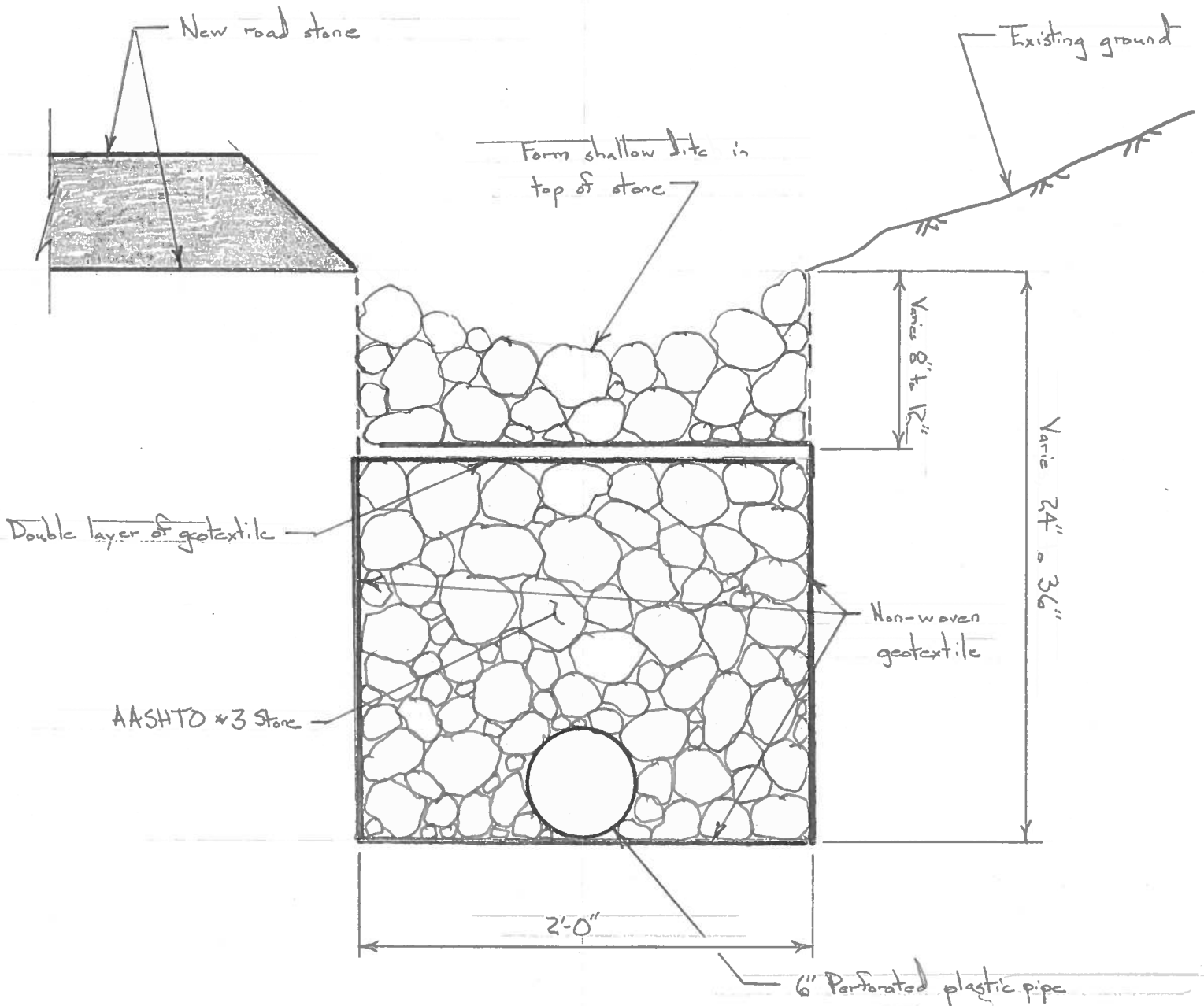
ATTACHMENT 4 UNDERDRAIN DETAIL Scale: 1 1/2 in. = 1 ft.
